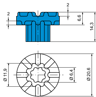
Bagues
